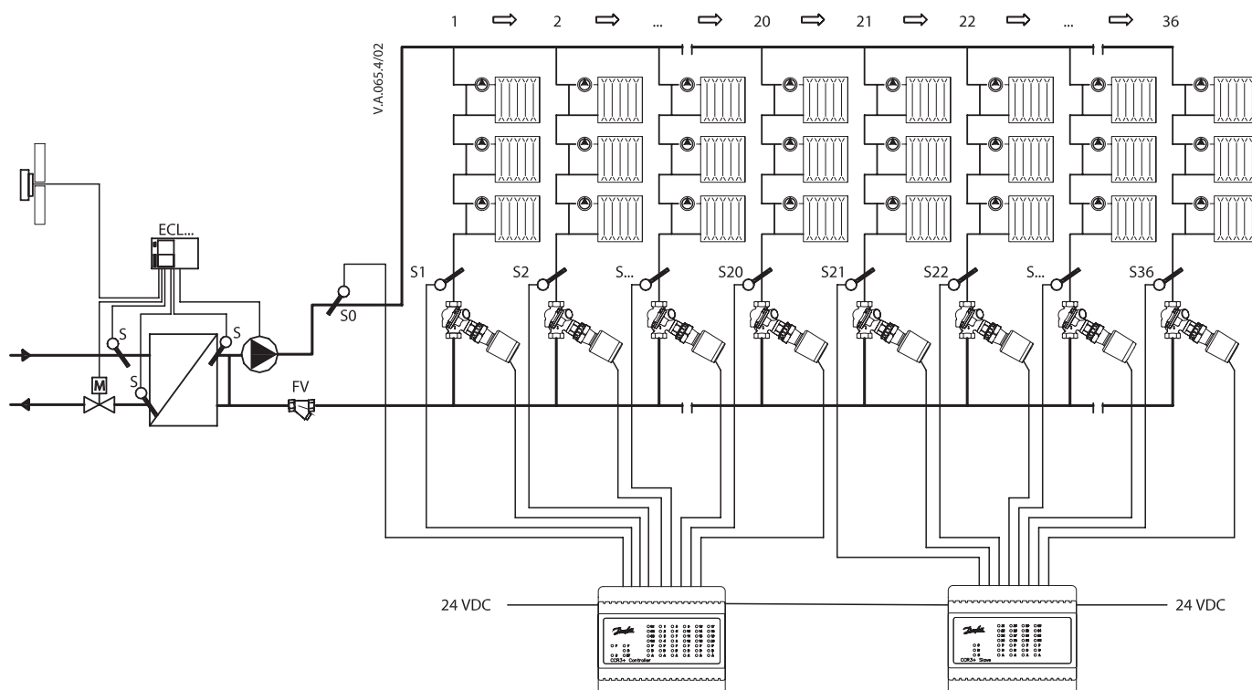
Fig. 2 Installation with CCR23 Controller (Master) and CCR+ Slave Unit (more that 20 risers)
